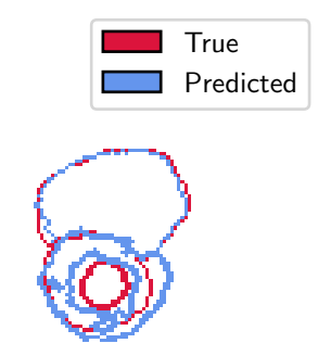
segmentations
